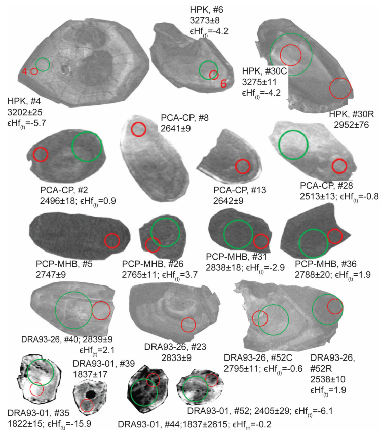
Figure 2. Representative CL images of analyzed zircon. Red smaller circles represent 20 \mu m U-Pb analysis spots. Green larger circles represent 40 \mu m Lu-Hf analysis spots.
