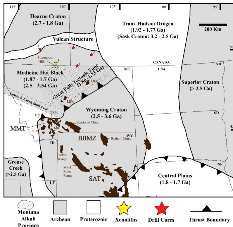
Figure 1. Generalized map of Precambrian basement provinces of southwestern Laurentia with the Montana alkali province (MAP) shown without a solid boundary, as the extent of the MAP is not well known (after [2,15–19]). MMT: Montana Metasedimentary Terrane; BBMZ: Bighorn-Beartooth Magmatic Zone. TRM: Tobacco Root Mountains; HM: Highland Mountains; RR: Ruby Range; MR: Madison Range; LRM: Little Rocky Mountains; LBM: Little Belt Mountains. Drill core locations: (1) Home Pacific Knappen; (2) Imperial Calstan Lake Newell; (3) PCA Calstan Parkland; (4) PCP Medicine Hat. Xenolith localities: (5) Coulee 29; (6) Sill 39.
