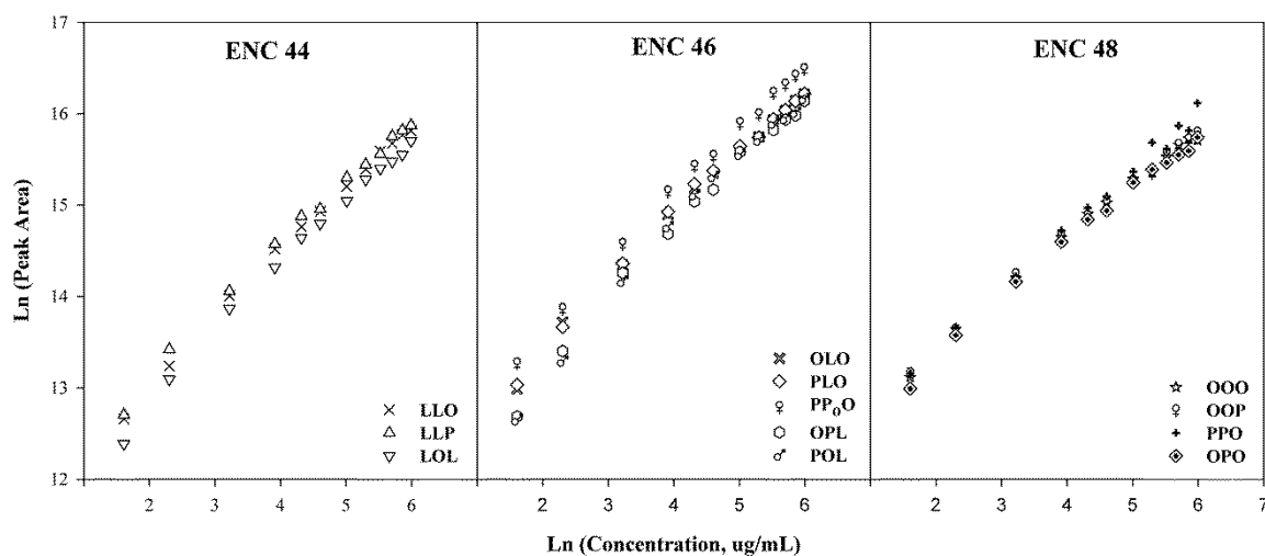
Figure 6. Calibration curves (grouped by ECN) for 12 commercially available reference standards.
