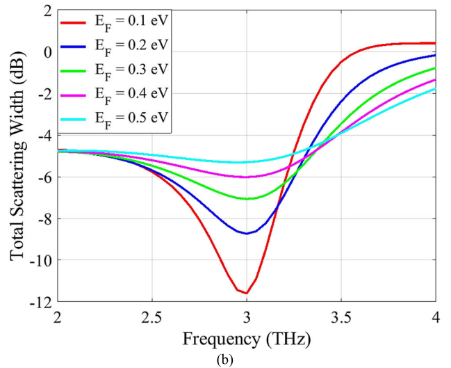
FIGURE 14. Frequency dispersion of the total SW and (b) SW versus frequency, showing tunability in magnitude of cloaking for an elliptical PEC cylinder cloaked by graphene-metal metasurface for \tau = 20 fs.
