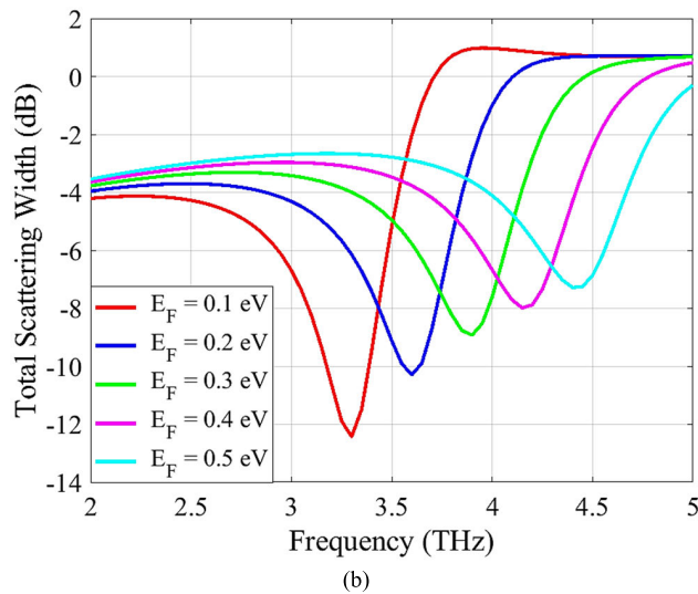
FIGURE 12. (a) Frequency dispersion of the total SW and (b) SW versus frequency, showing tunability in cloaking frequency for an elliptical PEC cylinder cloaked by graphene-metal metasurface for \tau = 200 fs.
