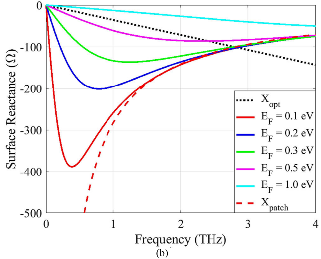
FIGURE 10. SW versus frequency for a cloaked circular PEC cylinder, showing tunability in magnitude of cloaking, and (b) frequency dispersion of the surface reactance for different Fermi energy ( E_F ).
