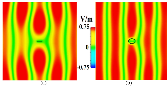
FIGURE 17. Snapshots of the electric field distribution for (a) uncloaked and (b) cloaked 2D PEC strip impinged by a TM-polarized plane wave at normal incidence for \tau = 200 fs.
