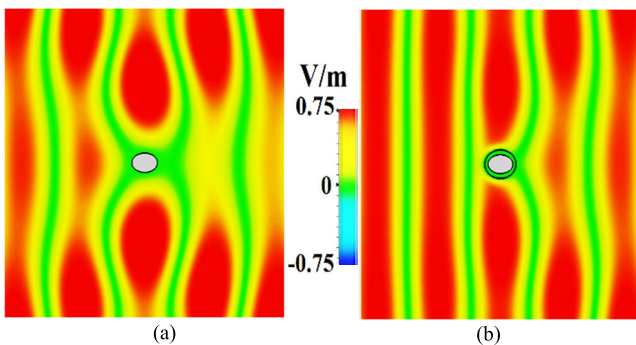
FIGURE 13. Snapshots of the electric field distribution for (a) uncloaked, and (b) cloaked elliptical cylinder impinged by a TM-polarized plane wave at normal incidence for \tau = 200 fs.
