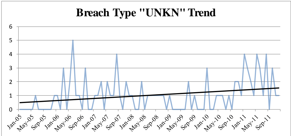
Figure 21 - "Unknown" Trend
