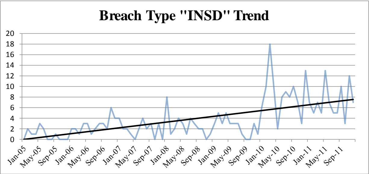
Figure 7 - "Insider" Trend
