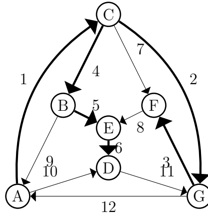
FIGURE 1.6. The Pyramid Graph
