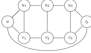
FIGURE 2.2. The Graph V_4
