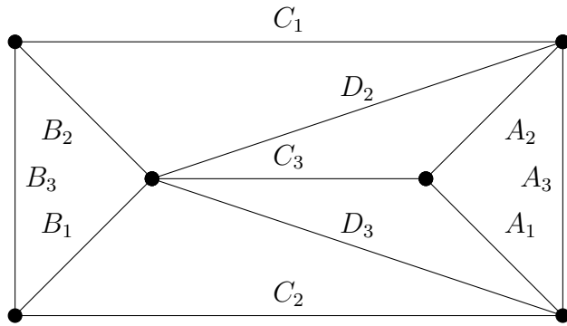
Figure 3.9: Another labeled extensions of the Prism graph
