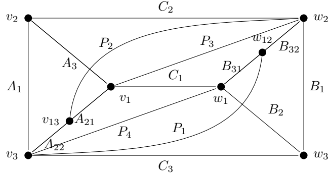
Figure 2.27: The graph \text{Prism}^{\perp\perp++}
