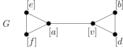
Figure 7: Bridge Theorem Example
