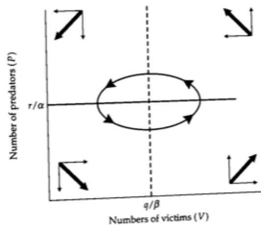
Lotka-Volterra Predation Model
