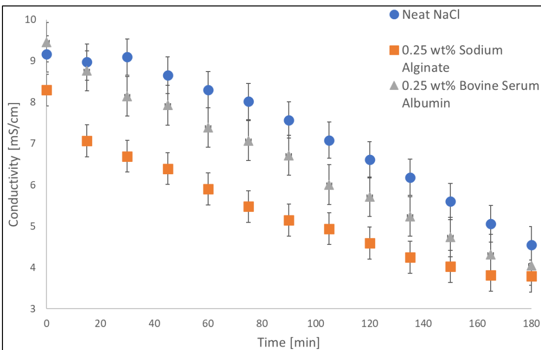
Figure 3-2. Comparison of neat NaCl solution, 0.25 wt% added sodium alginate, 0.25 wt% bovine serum albumin with standard errors.
